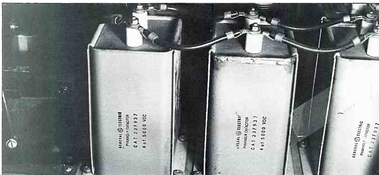
These Pyranol-filled capacitors were found in a circa 1962 10kW transmitter. Pyranol is General Electric's trade name for a PCB dielectric.
