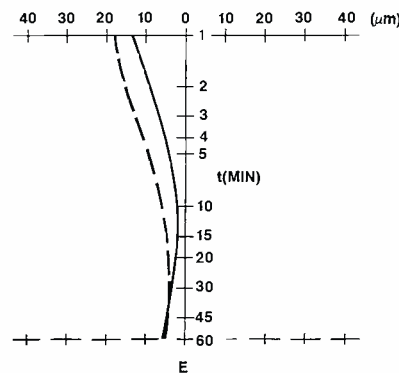
Figure 4. Spot displacement vs. time of a 66cm corner-pin tube (shown by solid lines), compared with its conventional counterpart (depicted by dashed lines).
