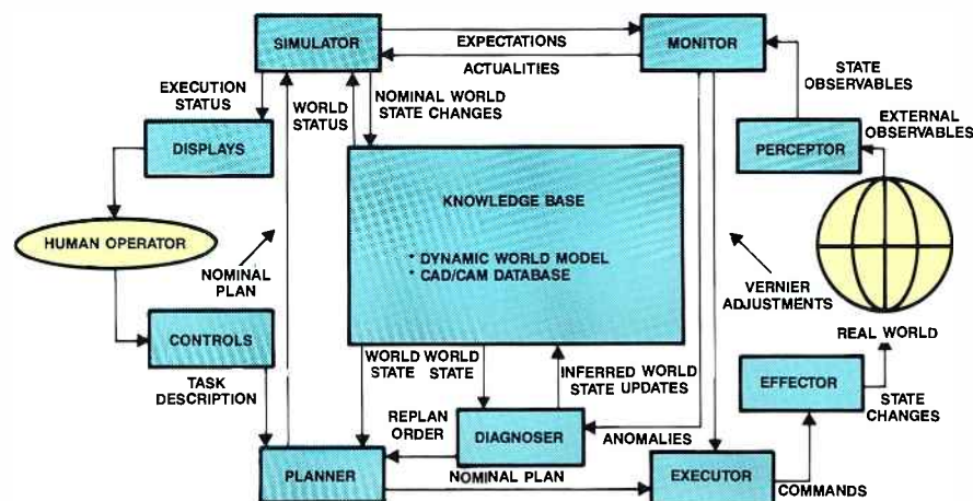
Figure 1. An overview of the intelligent autonomous system.
