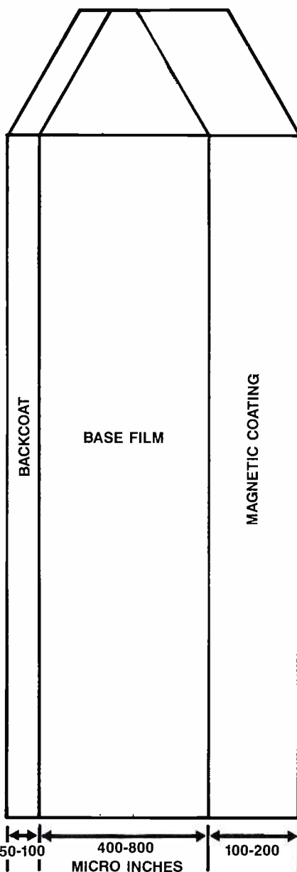
Figure 1. Videotape consists of a base film, a magnetic coating and a backcoat that protects the base film and dissipates static.
